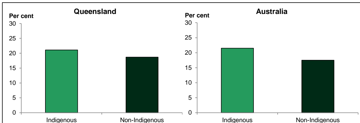
Figure 2.06.1: Proportion aged 15 and over who were currently studying, by Indigenous status, Queensland and Australia, 2014–15
